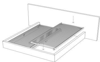
BED WITH HEADBOARD
