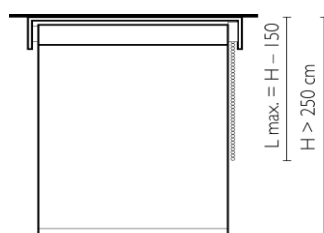
CHAIN LENGTH
