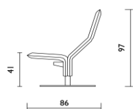
SWIVEL K CHAIR
